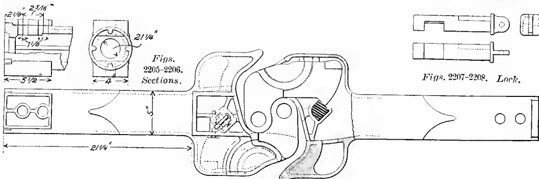
Fig. 2204. Plan of Couplers Locked.
